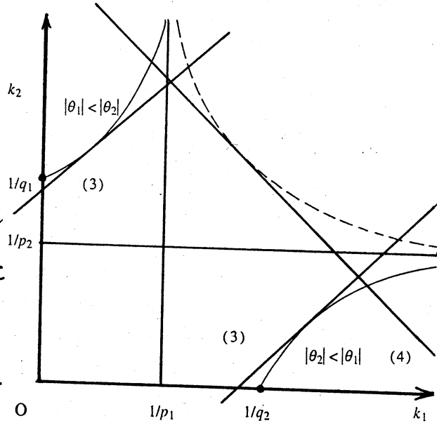
Fig. 3. Relations between r_1 and r_2 . Fig. 4. Relations between k_1 and k_2 .
